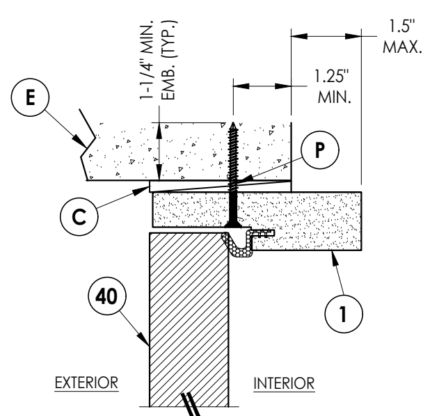
6 VERTICAL CROSS SECTION
